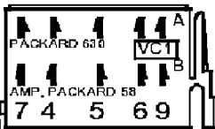
MARKING DETAIL REAR VIEW
