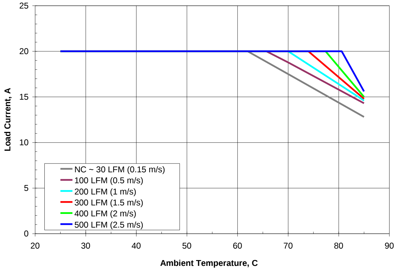
Figure 1. Available load current vs. ambient air temperature and airflow rates for SSQE48T20033 converter mounted vertically with air flowing from pin 1 to pin 3, V_{in} = 48\text{ V} . Note: NC – Natural convection
