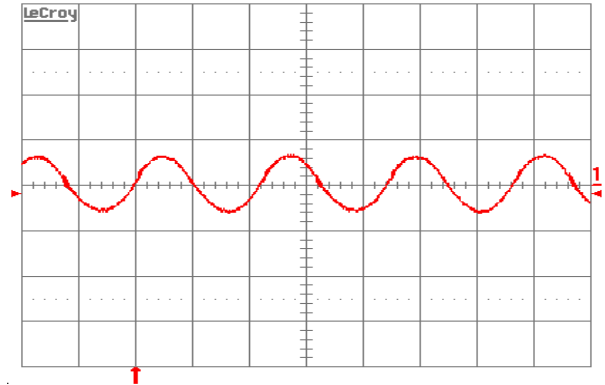
Figure 13. Input reflected ripple-current, i_c (200 mA/div.), measured at input terminals at full rated load current and V_{in} = 48 \text{ V} . Refer to Figure 11 for test setup. Time scale: 1 \mu\text{s}/\text{div} .
