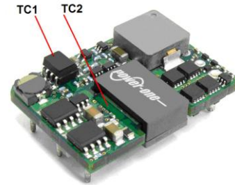
Fig. H: Locations of the thermocouple for thermal testing.
