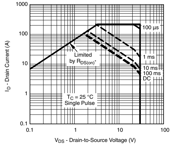
* V_{GS} > \text{minimum } V_{GS} \text{ at which } R_{DS(on)} is specified Safe Operating Area
