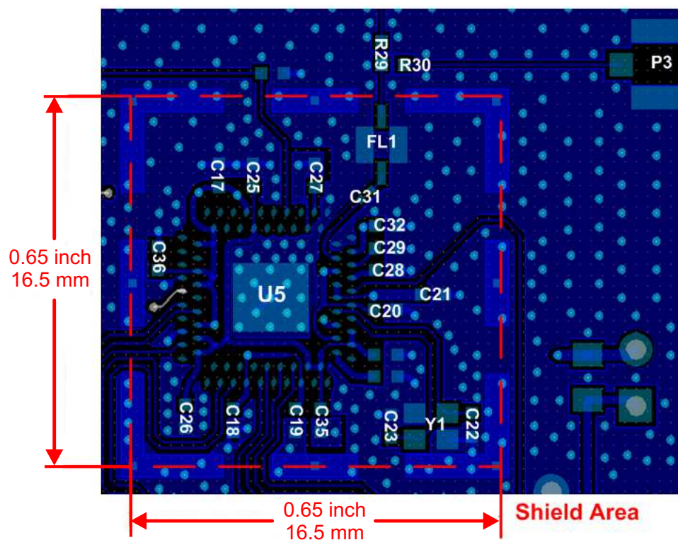
Figure 3. Component Placement
