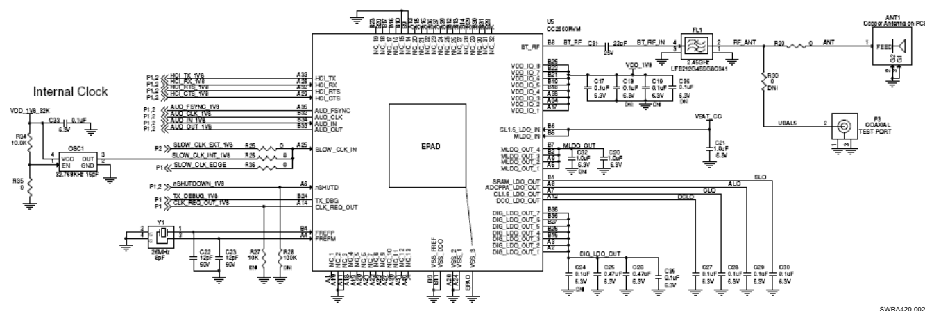
Figure 2. Reference Design Schematic
