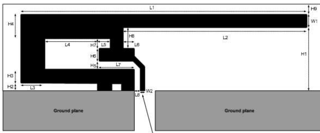
Figure 9. Inverted F Antenna Dimensions
