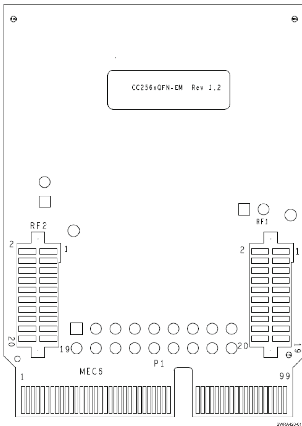
Figure 18. CC256x QFN EM Board – Bottom Side Mirror
