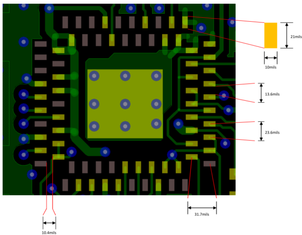
Figure 16. PCB Footprint
