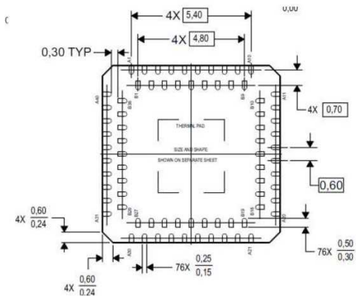
Figure 15. QFN Package Dimensions
