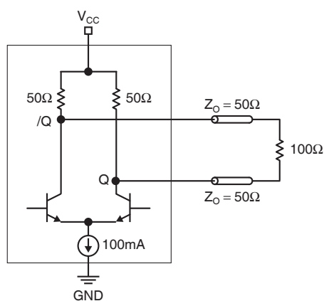
Figure 2b. CML DC-Coupled ( 100\Omega Termination)
