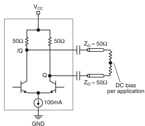
Figure 2c. CML AC-Coupled ( 50\Omega Termination)
