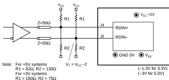
Figure 2. Test Set-Up
