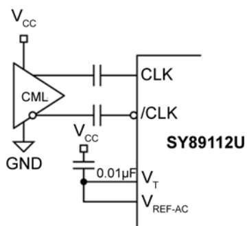
Figure 3d. CML Interface (AC-Coupled)
