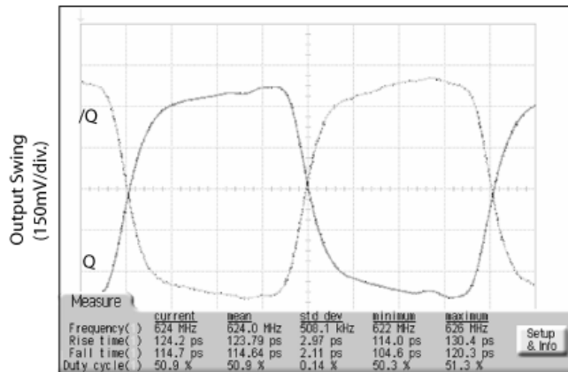
622MHz Output
