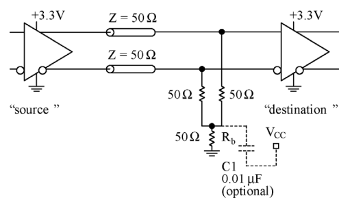
Figure 5. Three-Resistor "Y-Termination"
