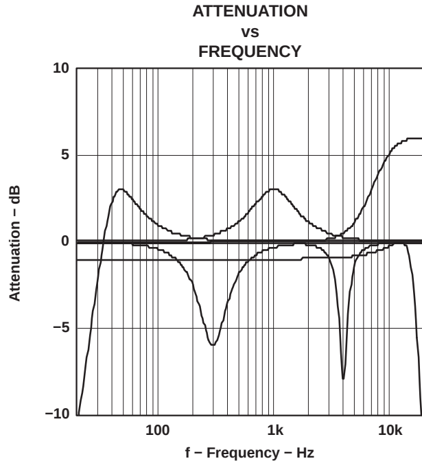
Figure 8-7. Individual Filters
