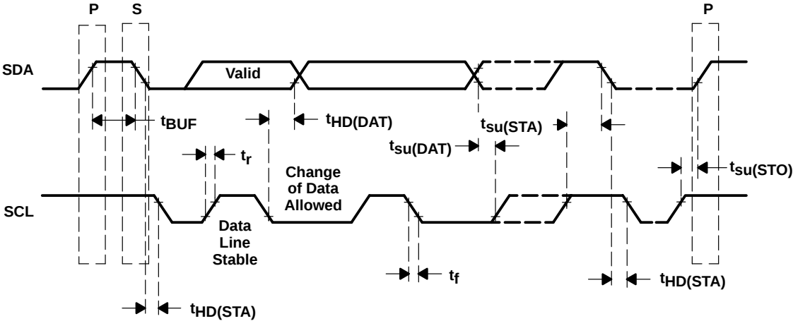
Figure 8–7. I 2 C Bus Timing
