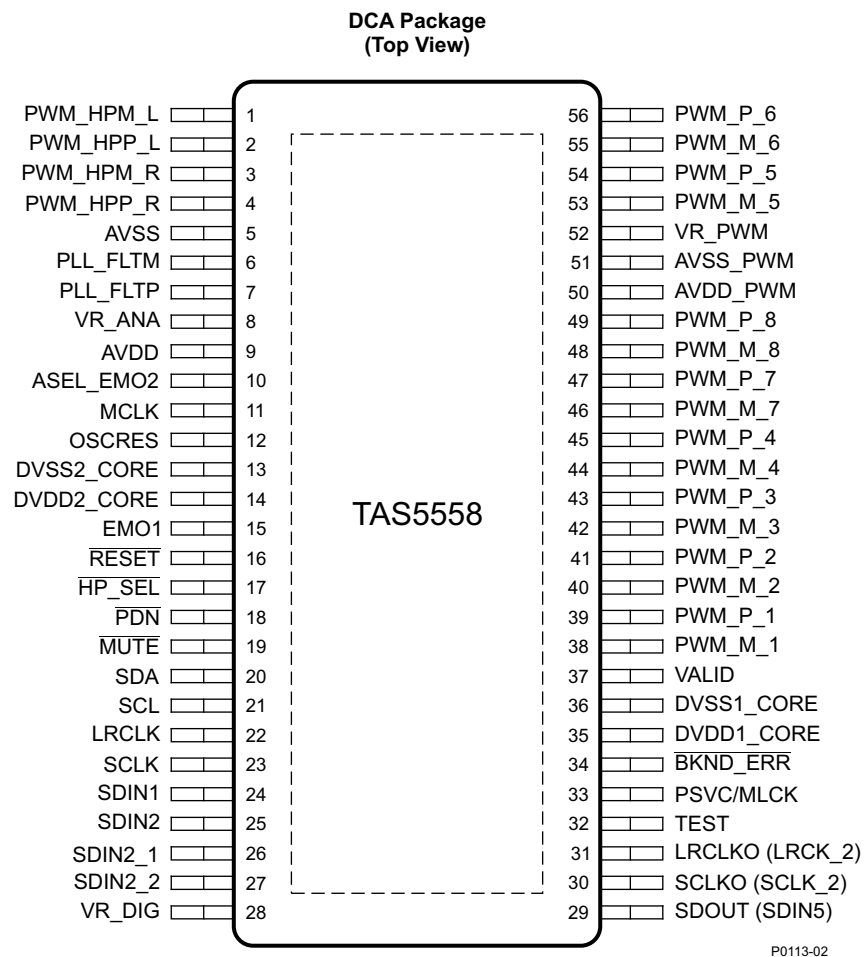
Figure 2-1. TAS5558 Pinout
