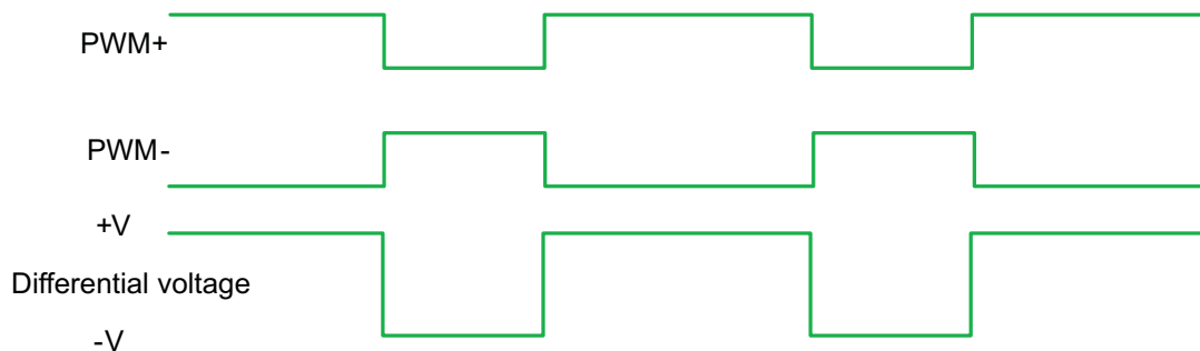
Figure 2-2. AD Modulation
