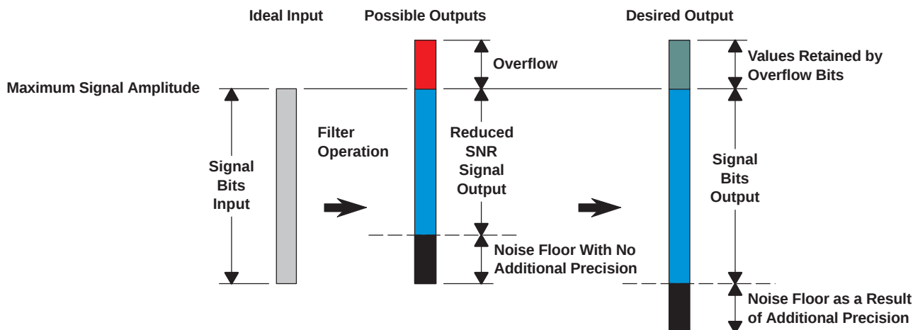
Figure 3-10. TAS5558 Digital Audio Processing
