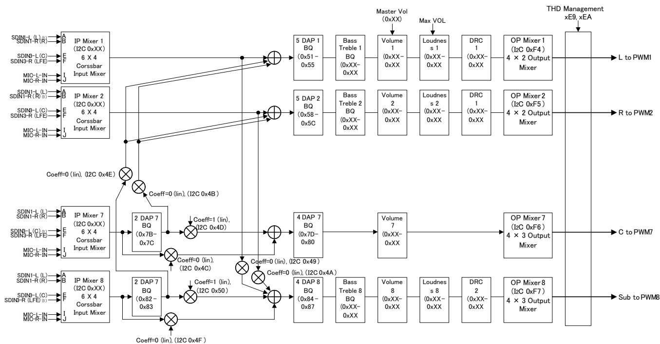
Figure 3-2. TAS5558 Architecture With I 2 C Registers in 192kHz Native Mode ( f_s = 176.4 kHz or f_s = 192 kHz)
