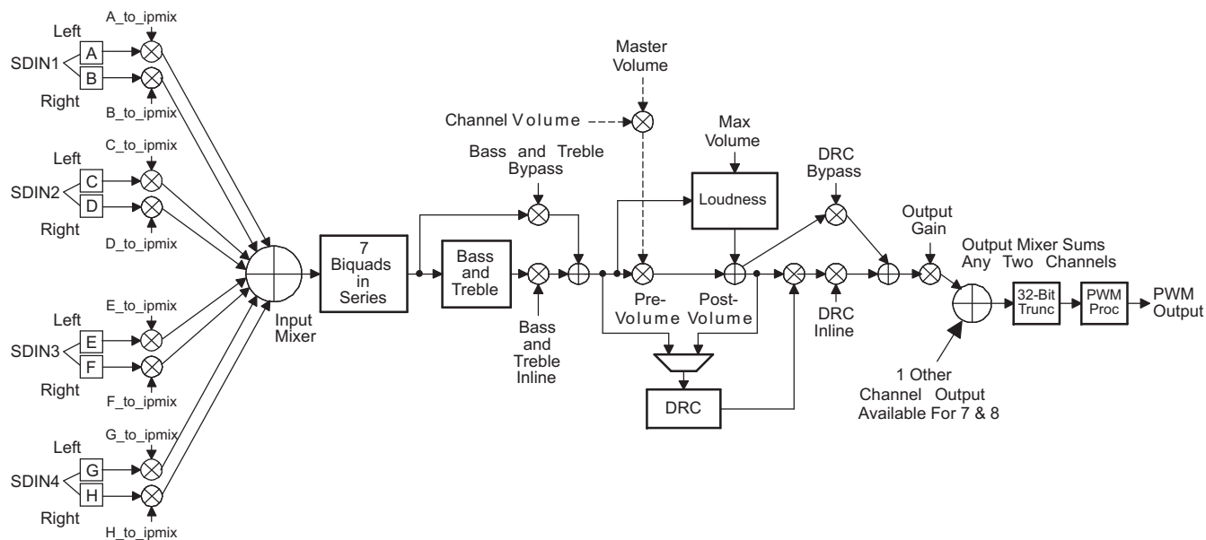
Figure 3-3. TAS5558 Detailed Channel Processing
