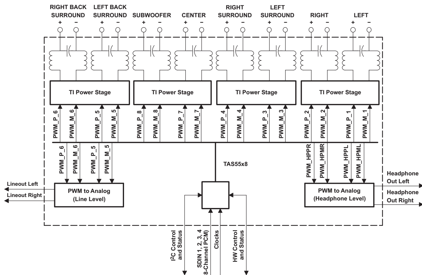
Figure 9-2. Pass-Through Output Mixer TAS5558 Channel Configuration
