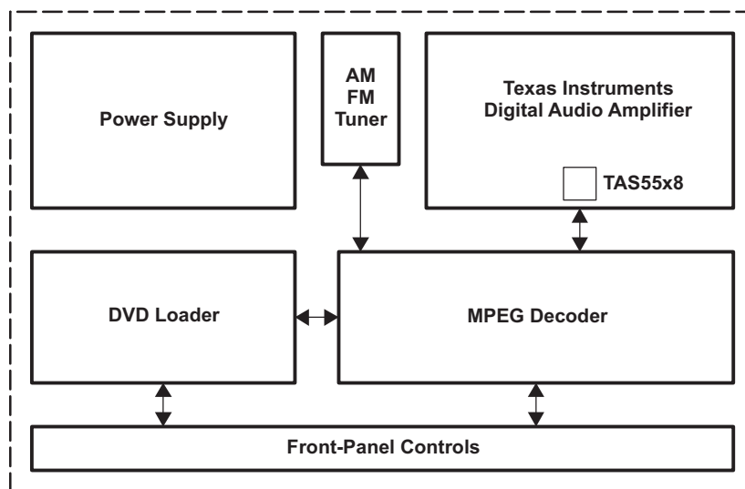
Figure 9-1. Typical TAS5558 Application (DVD Receiver)
