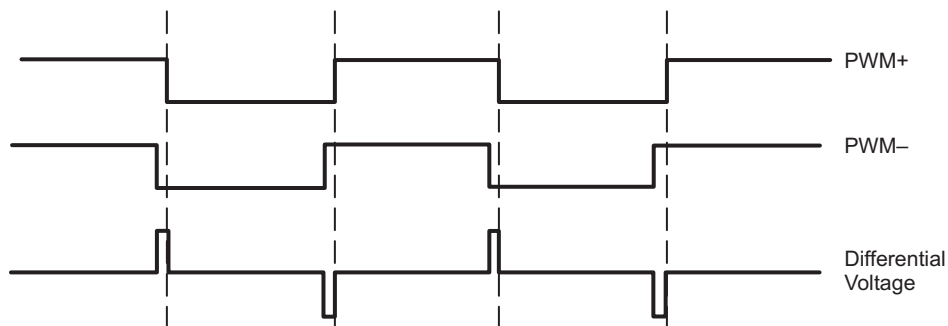
Figure 2-3. BD Modulation
