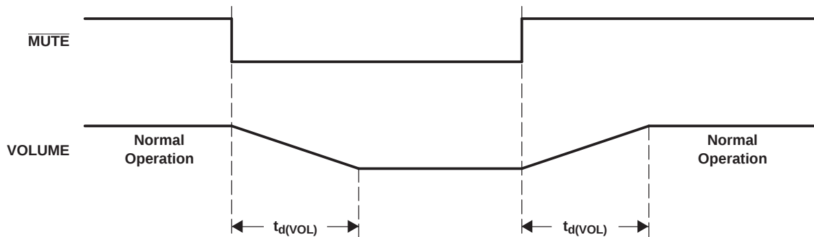
Figure 7-7. Mute Timing
