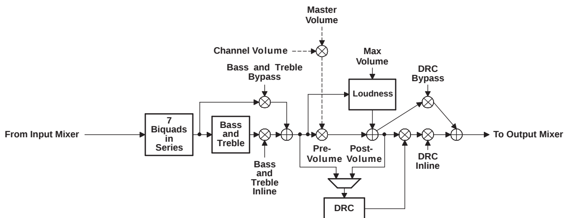
Figure 3-15. DRC Positioning in TAS5558 Processing Flow
