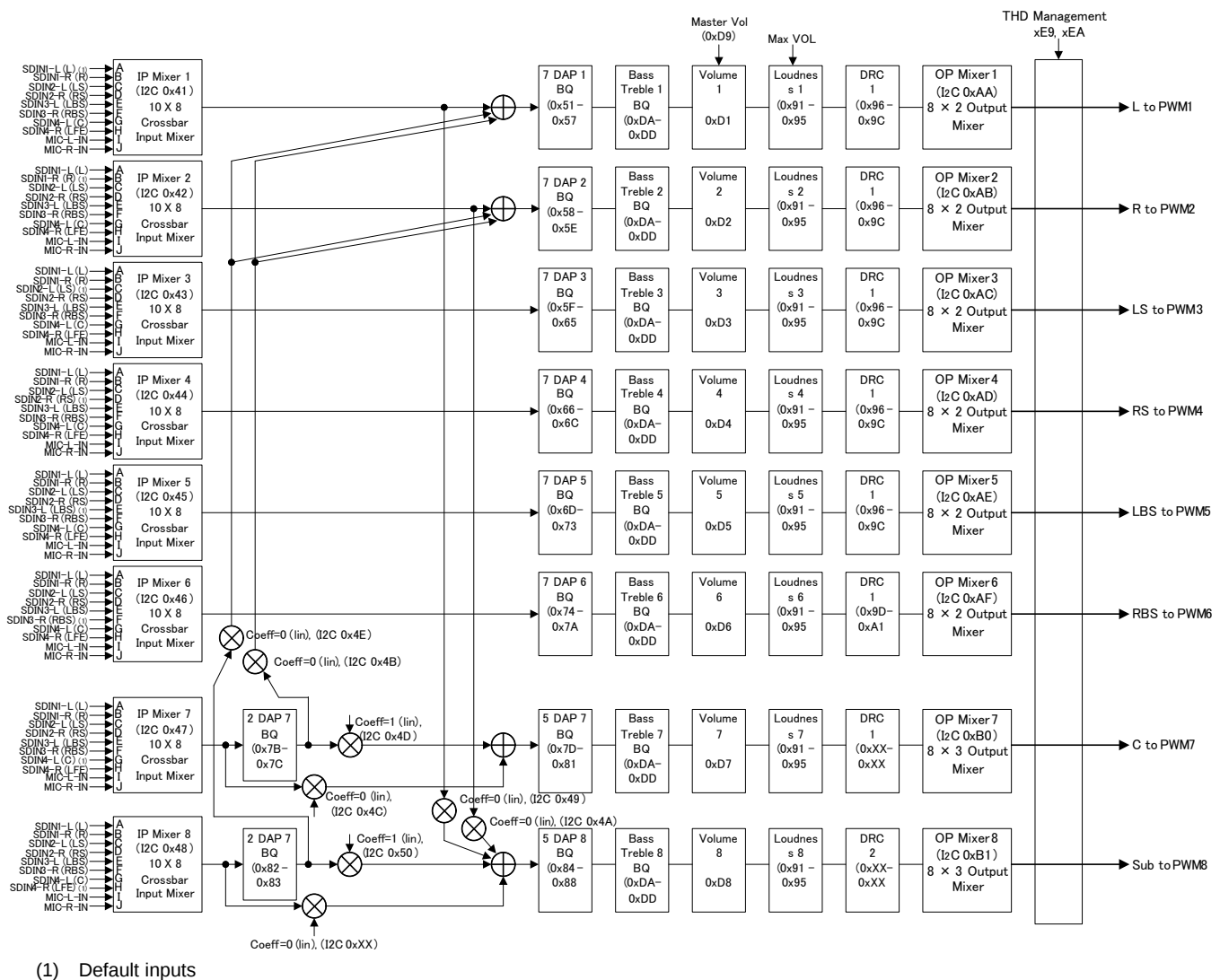
Figure 3-1. TAS5558 DAP Architecture With I 2 C Registers ( f_s \leq 96 kHz)
