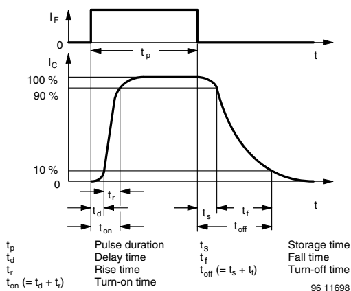
Fig. 11 - Switching Times
