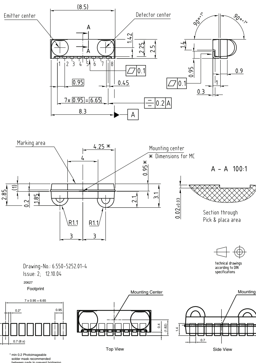
Fig. 8 - Package Drawing
