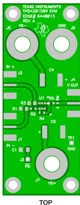
Figure 78. THS4281EVM Layout (Top Layer and Silkscreen Layer)
