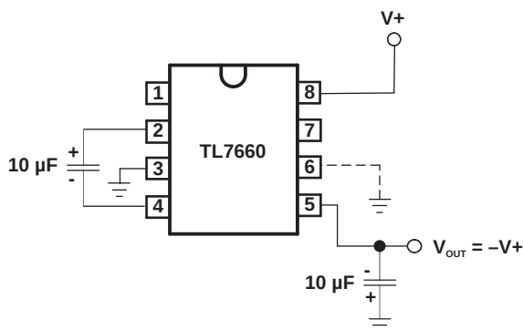
Figure 3. Simple Negative-Voltage Converter
