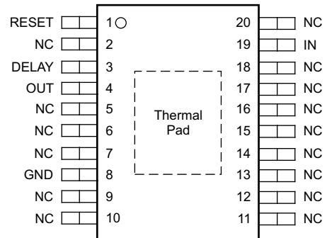
PWP (HTSSOP) Package (Top View)
