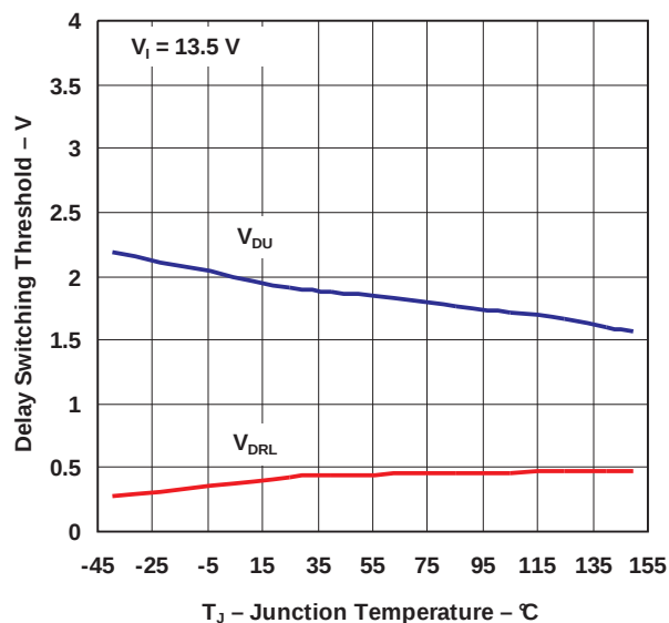
DELAY SWITCHING THRESHOLD versus JUNCTION TEMPERATURE
