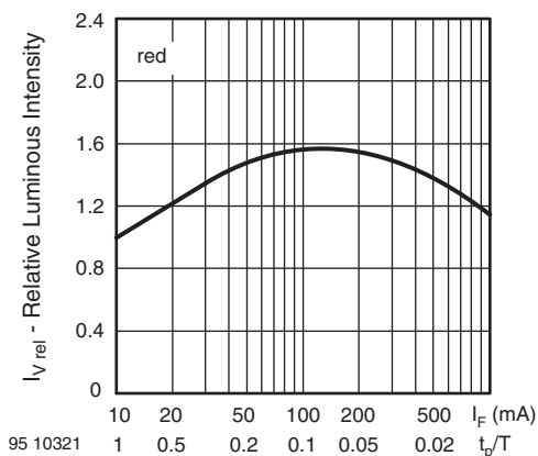
Fig. 8 - Relative Luminous Intensity vs. Forward Current/Duty Cycle
