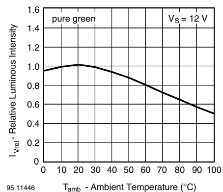
Fig. 28 - Relative Luminous Intensity vs. Ambient Temperature
