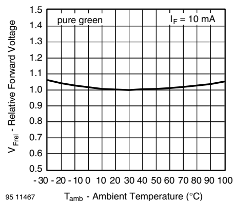
Fig. 26 - Relative Forward Voltage vs. Ambient Temperature
