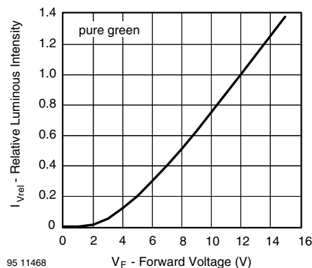
Fig. 27 - Relative Luminous Intensity vs. Forward Voltage
