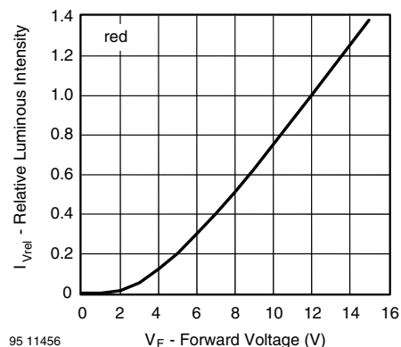
Fig. 4 - Relative Luminous Intensity vs. Forward Voltage
