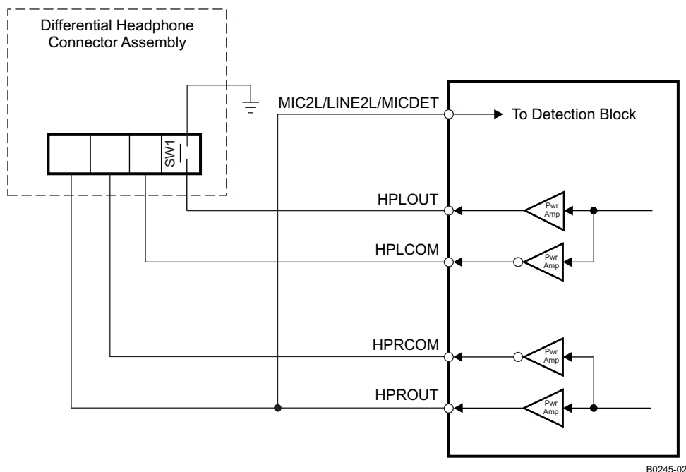
Figure 36. Configuration of Device for Jack Detection Using a Fully Differential Stereo Headphone Output Connection
