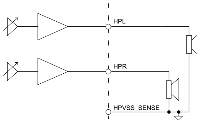
Figure 24. TLV320AIC3262 Ground-Centered Headphone Output
