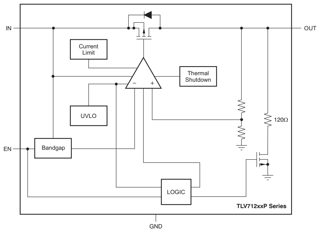
Figure 2. TLV712xxP
