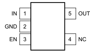
DBV PACKAGE SOT23-5 (Top View)
