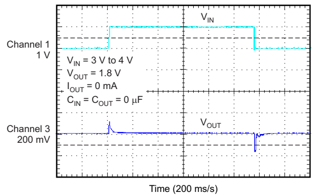
Figure 12. LINE TRANSIENT
