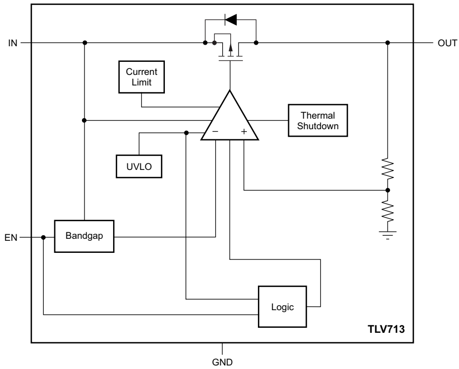
Figure 1. TLV713 Block Diagram
