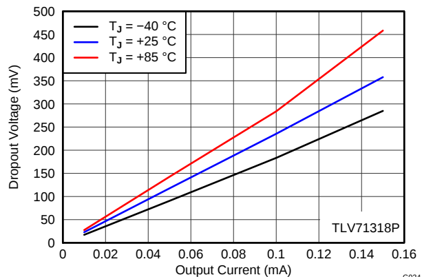
Figure 5. 1.8-V DROPOUT VOLTAGE vs I_{OUT} AND TEMPERATURE
