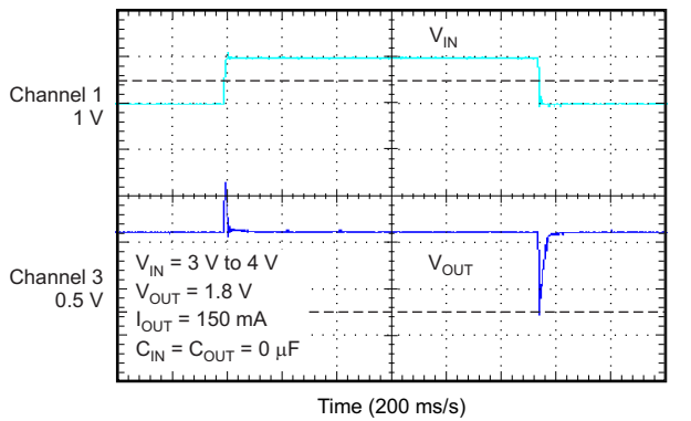
Figure 13. LINE TRANSIENT
