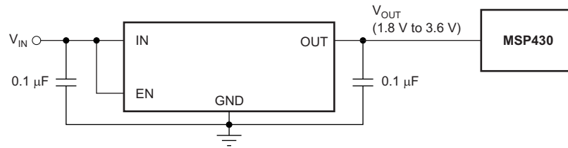
Figure 24. TLV713 Powering a Microcontroller
