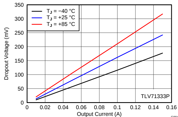
Figure 6. 3.3-V DROPOUT VOLTAGE vs I_{OUT} AND TEMPERATURE
