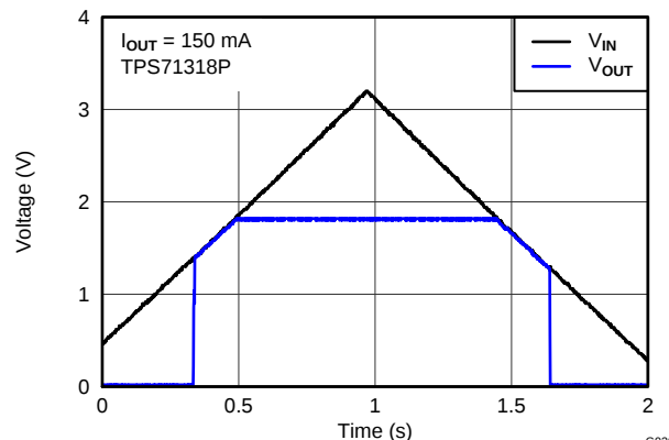
Figure 20. V_{IN} POWER-UP AND POWER-DOWN
