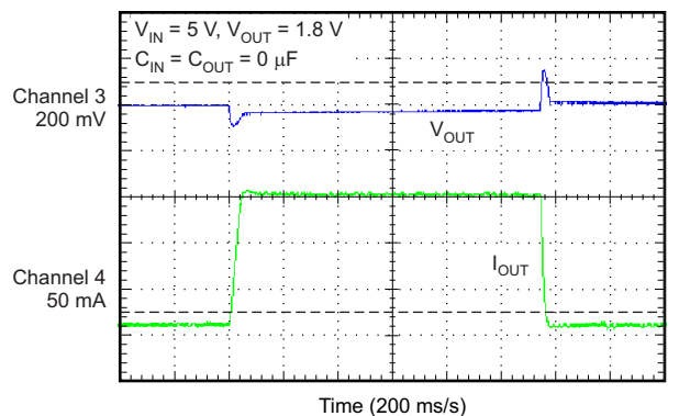
Figure 19. 10-mA to 150-mA LOAD TRANSIENT
