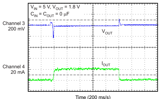
Figure 15. 0-mA to 20-mA LOAD TRANSIENT
