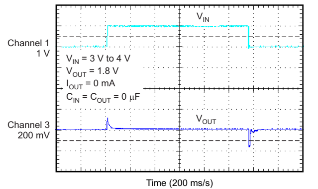
Figure 12. LINE TRANSIENT
