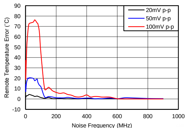
Figure 6. REMOTE TEMPERATURE ERROR vs REMOTE CHANNEL NOISE FREQUENCY
