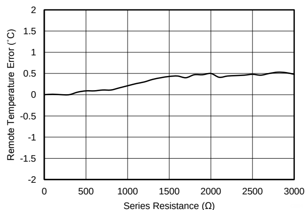
Figure 4. REMOTE TEMPERATURE ERROR vs SERIES RESISTANCE
