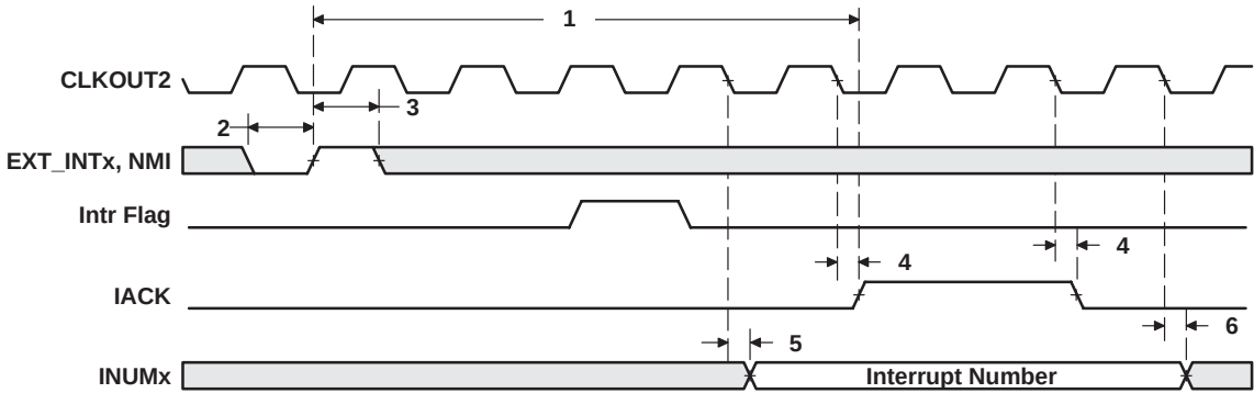
Figure 29. Interrupt Timing
