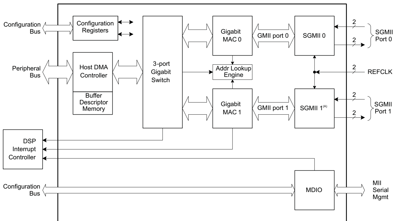
Figure 6-47. Ethernet Subsystem Block Diagram
