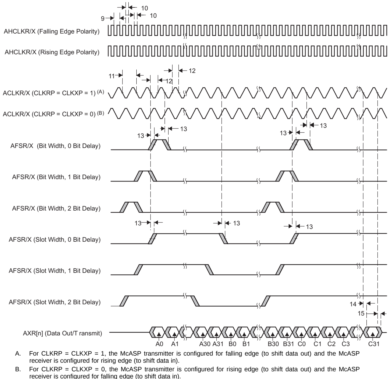
Figure 6-44. McASP Output Timing
