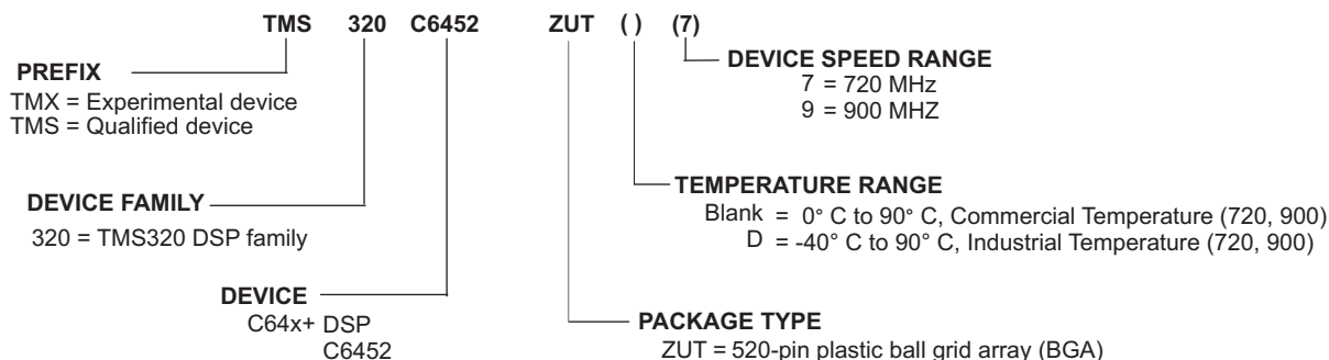
Figure 2-6. Device Nomenclature
