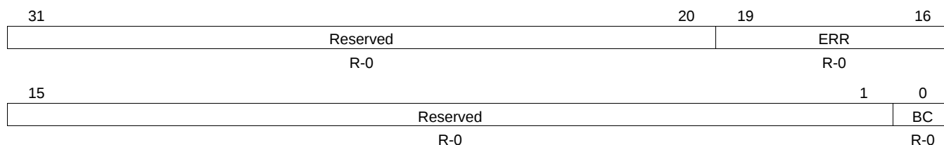
Figure 3-3. BOOTCMPLT Register 3
