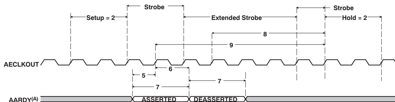
Figure 6-23. AARDY Timing
