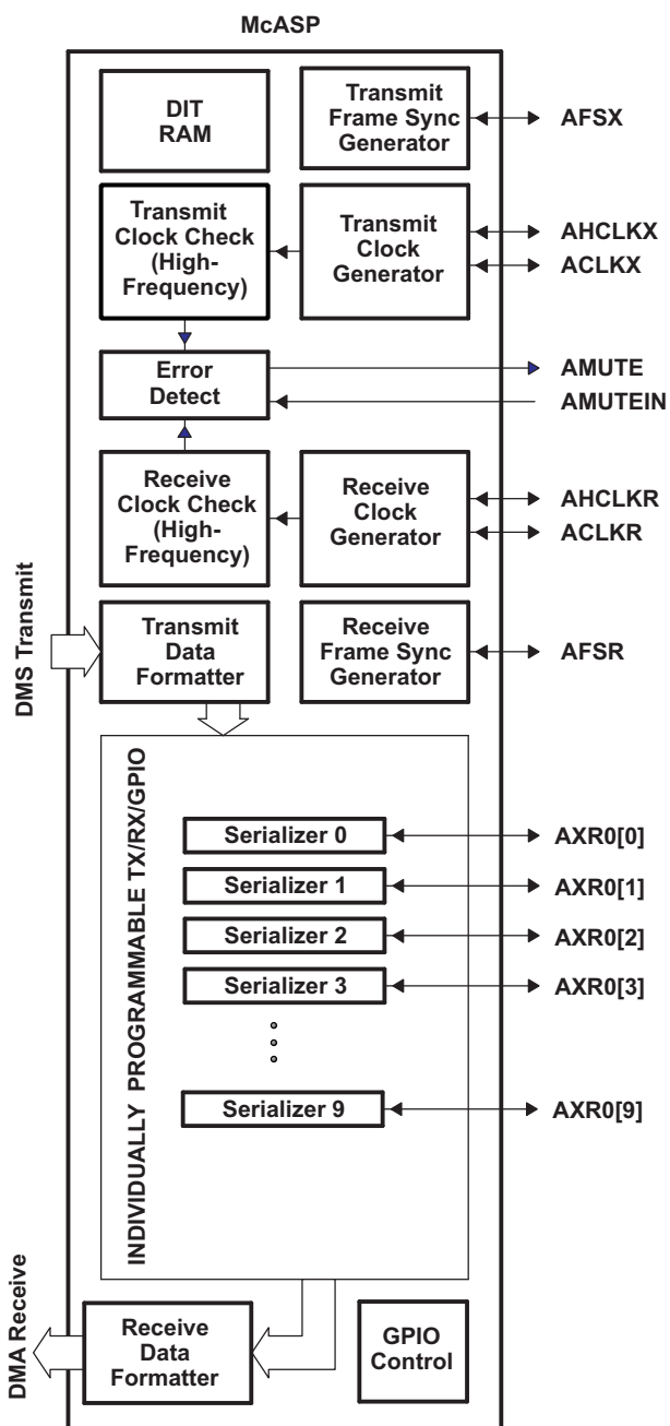
Figure 6-42. McASP Configuration
