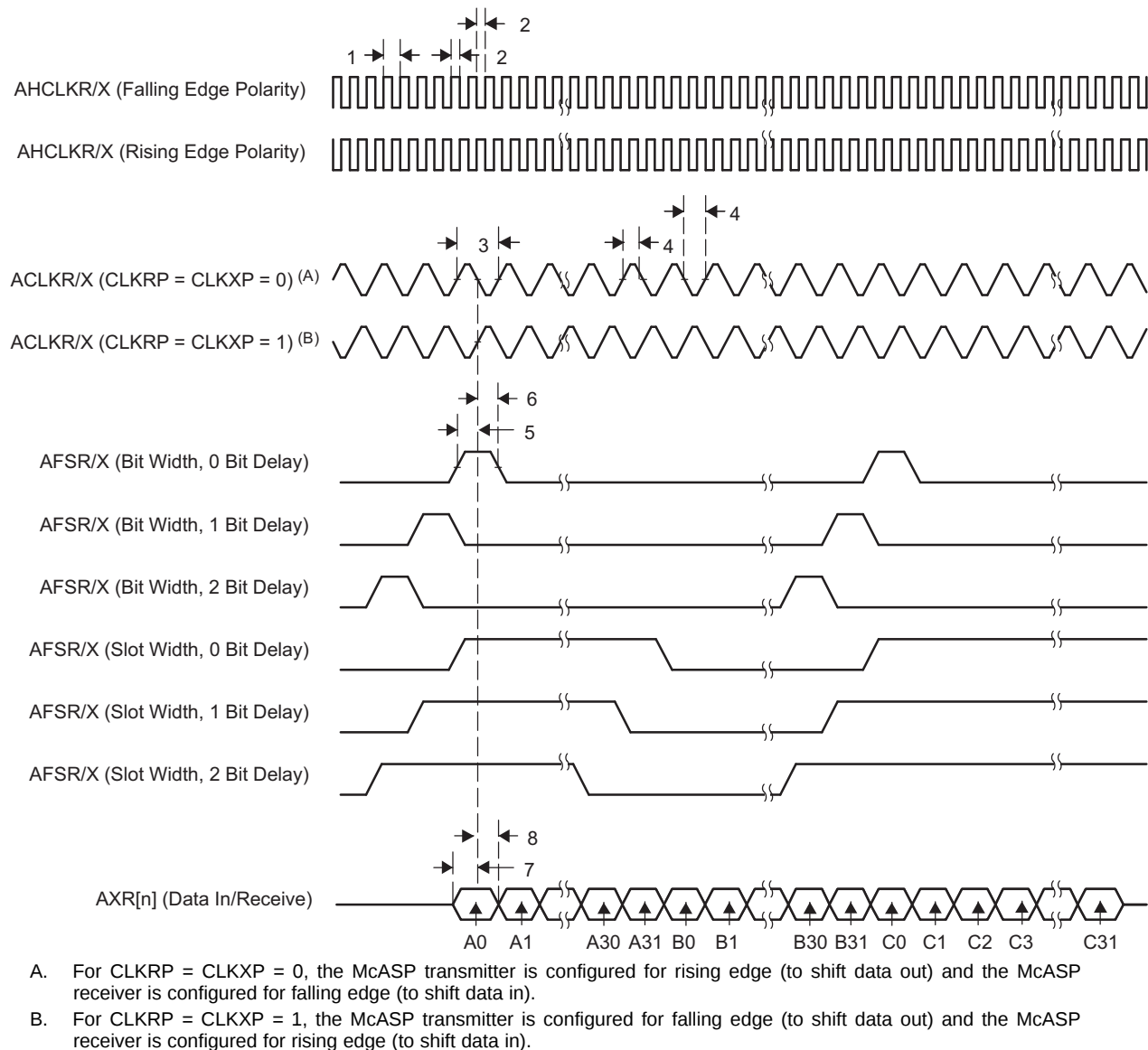
Figure 6-43. McASP Input Timing
