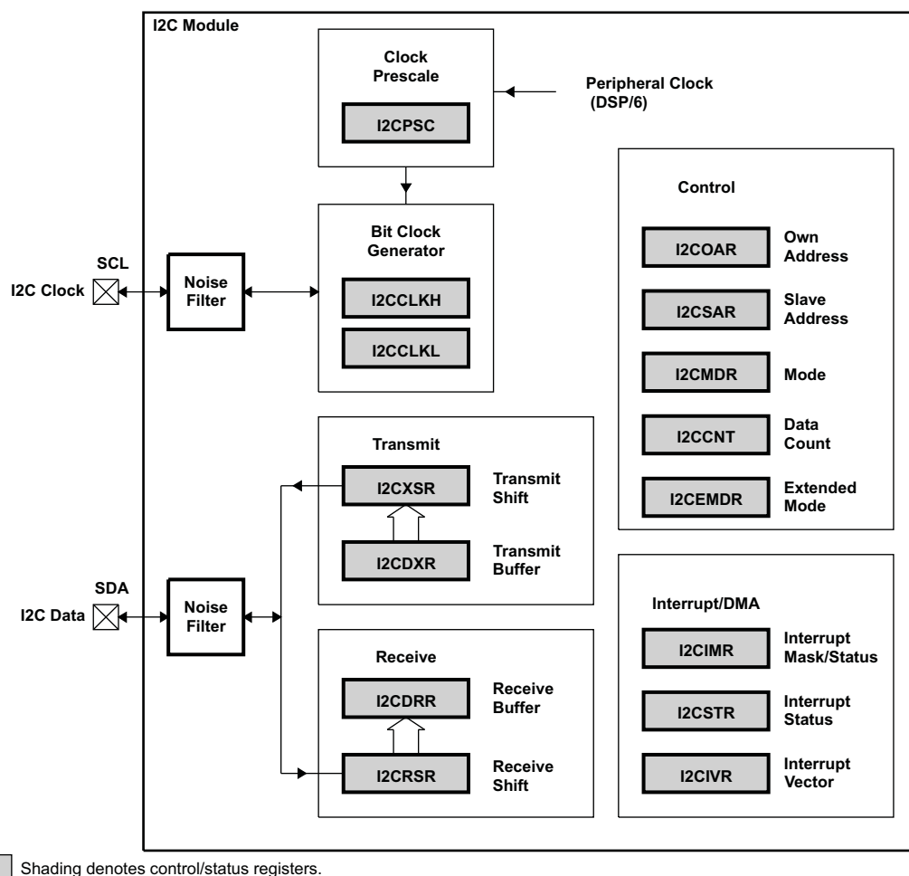
Figure 6-31. I2C Module Block Diagram
