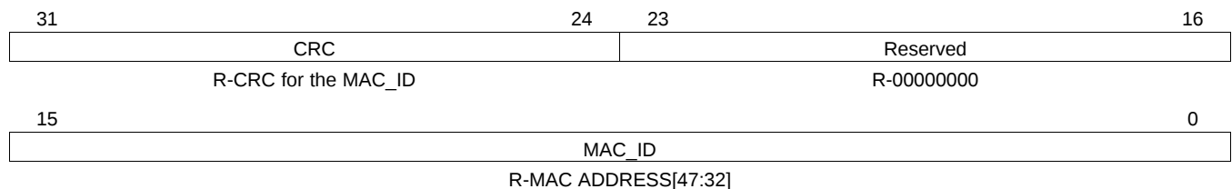
Figure 3-8. MAC_ADDR_R1 Register
