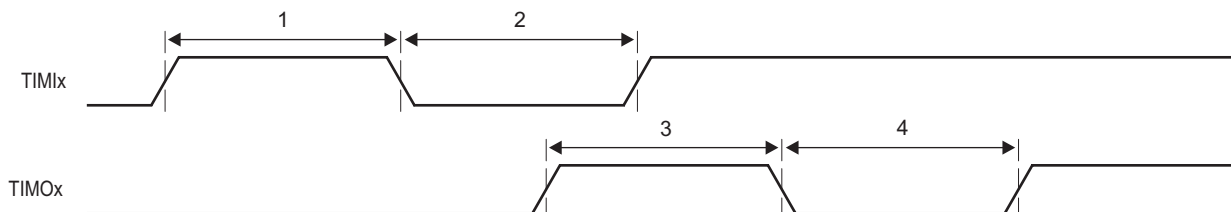
Figure 7-52 Timer Timing
