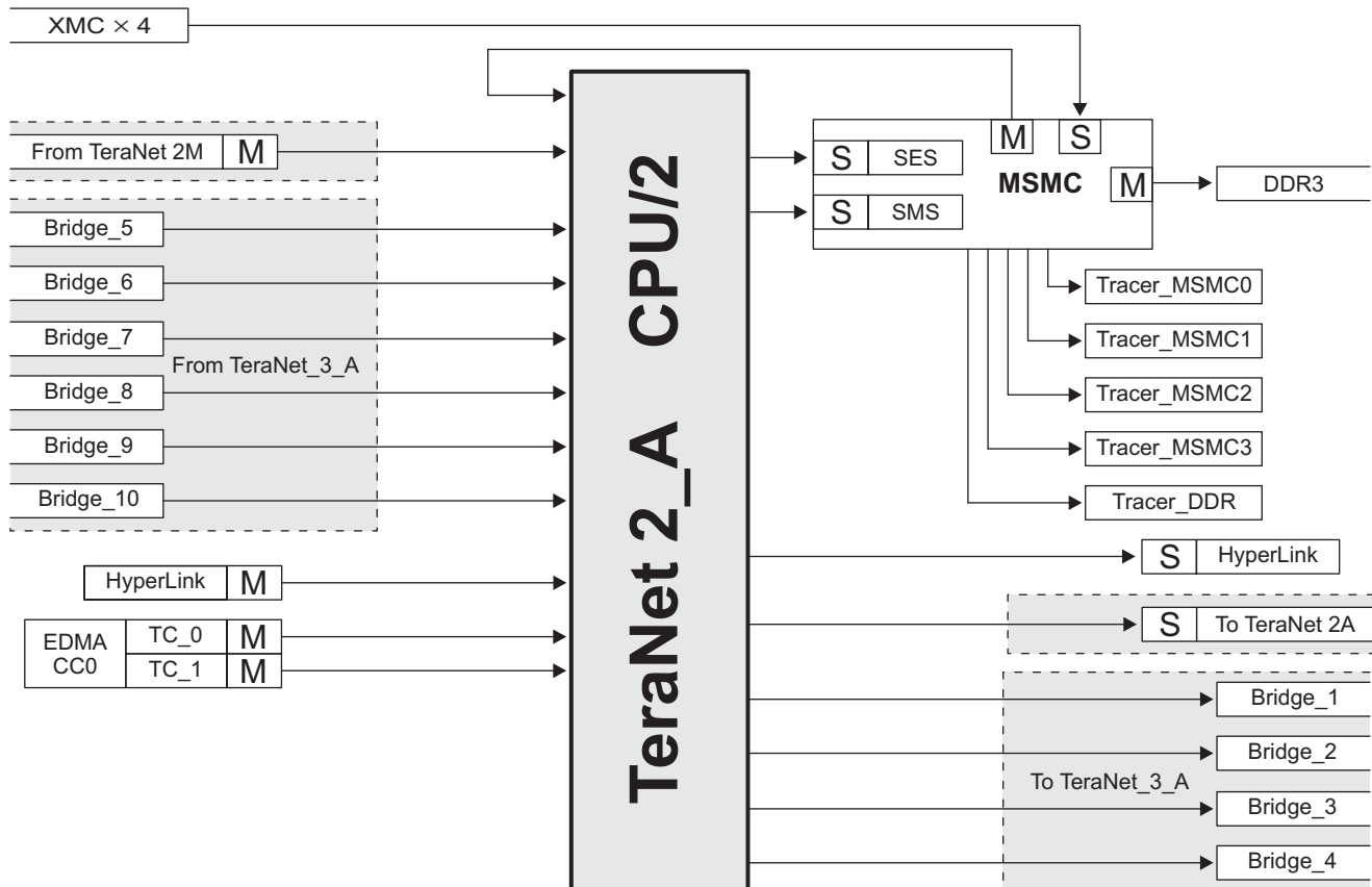
Figure 4-2 TeraNet 2A
