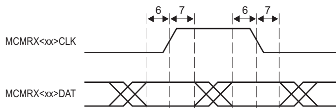
Figure 7-43 HyperLink Station Management Receive Timing
