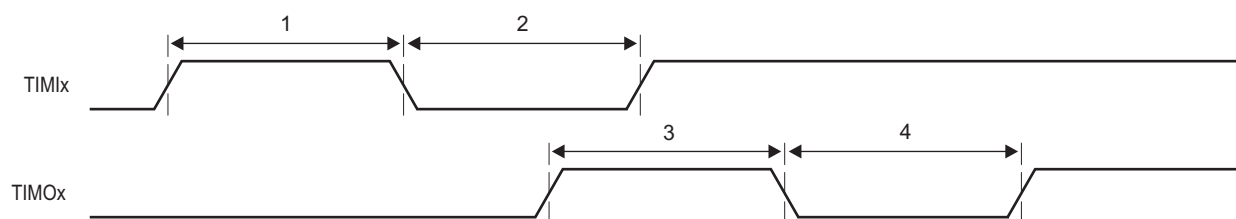
Figure 7-59 Timer Timing
