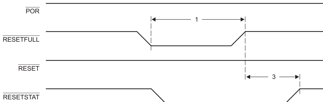
Figure 7-5 Soft/Hard-Reset Timing
