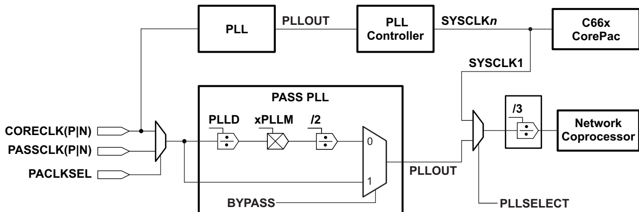
Figure 7-25 PASS PLL Block Diagram
