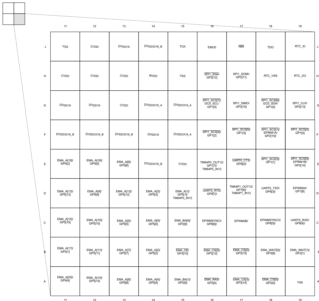
Figure 2-5. Pin Map (Quad C)
