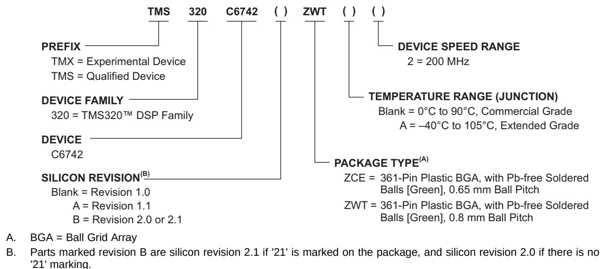
Figure 6-1. Device Nomenclature
