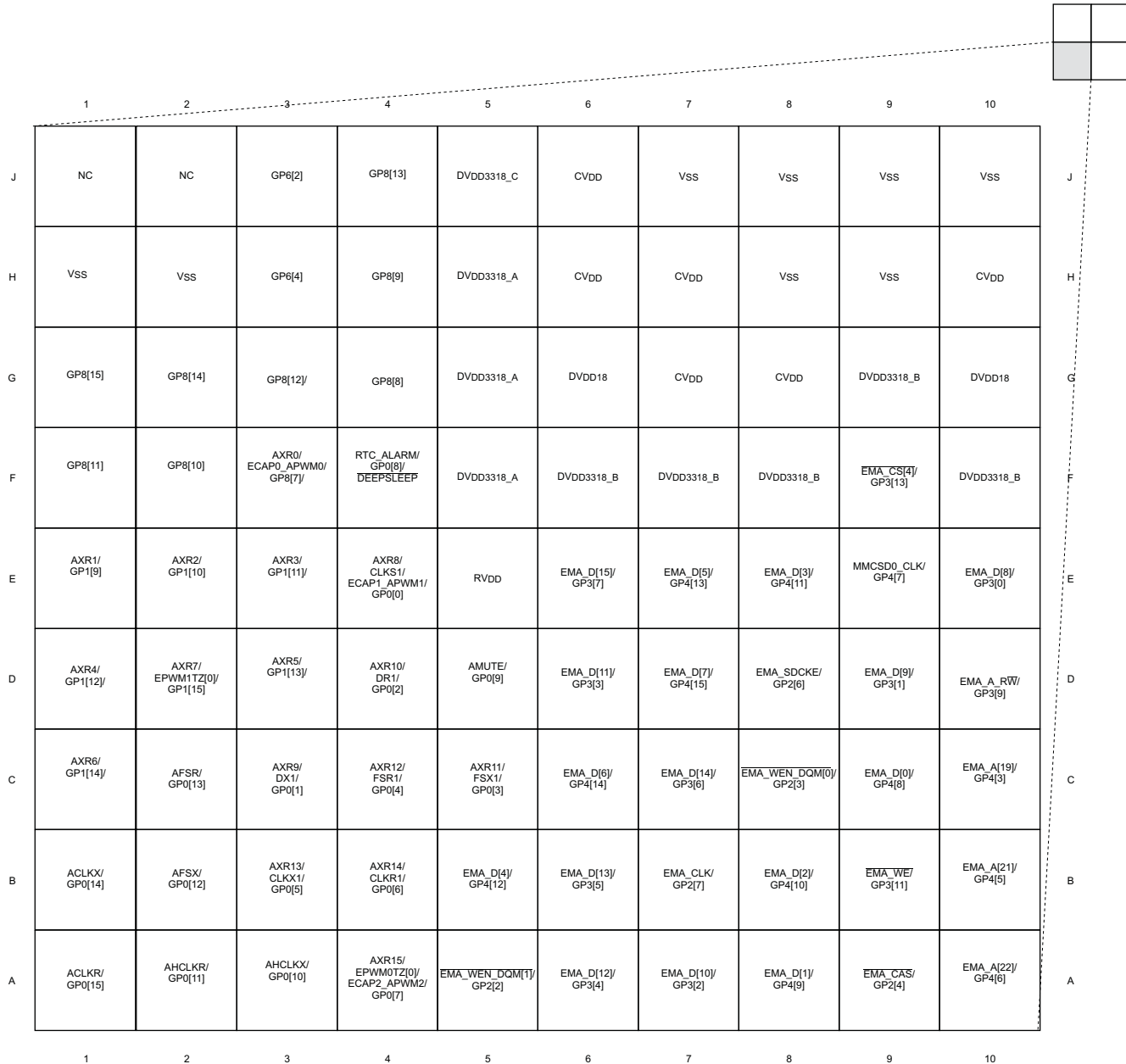
Figure 2-6. Pin Map (Quad D)
