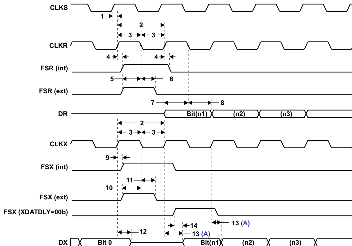
Figure 5-29. McBSP Timing
