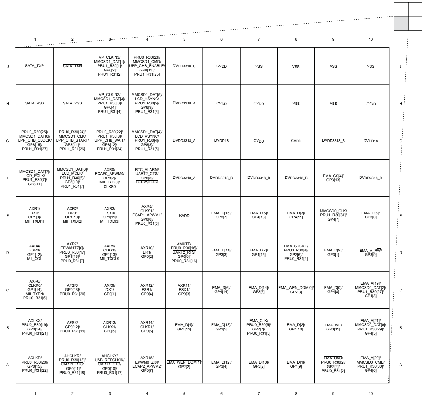
Figure 2-6. Pin Map (Quad D)
