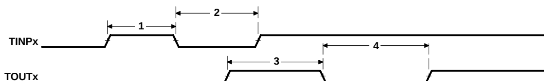
Figure 4-62. Timer Timing
