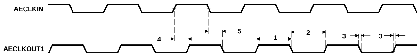
Figure 4–17. AECLKOUT1 Timing for the EMIFA Module
