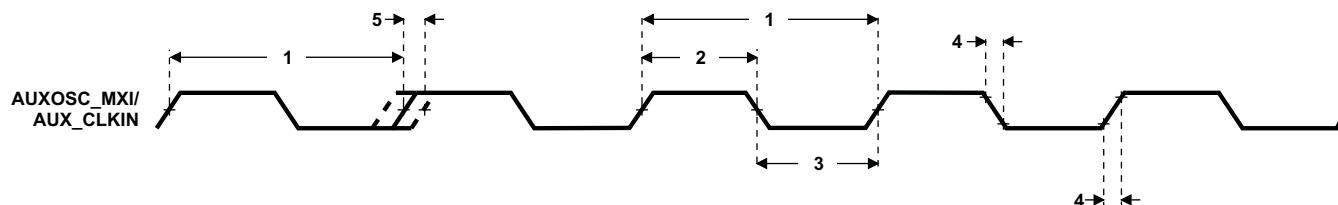
Figure 7-13. AUX_MXI/AUX_CLKIN Timing
