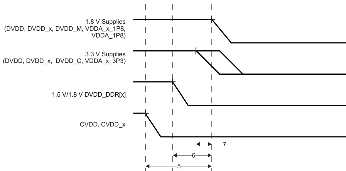
Figure 7-3. Power-Down Sequence
