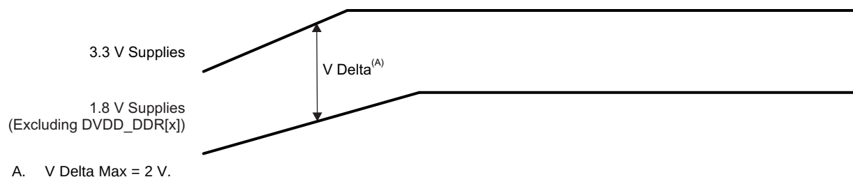
Figure 7-2. 3.3 V Supplies Rising Before 1.8 V Supplies Delta
