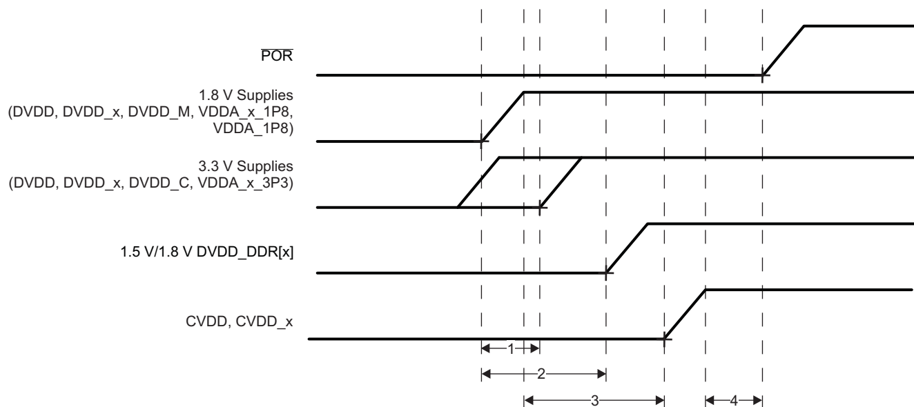
Figure 7-1. Power-Up Sequence
