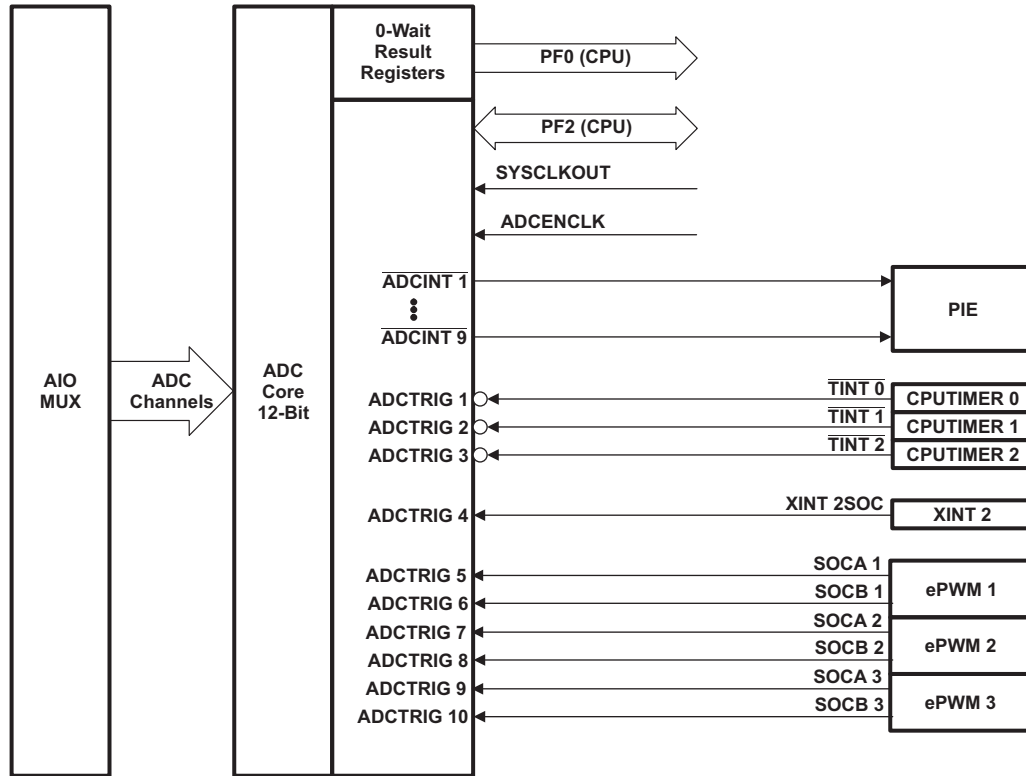
Figure 6-3. ADC Connections
