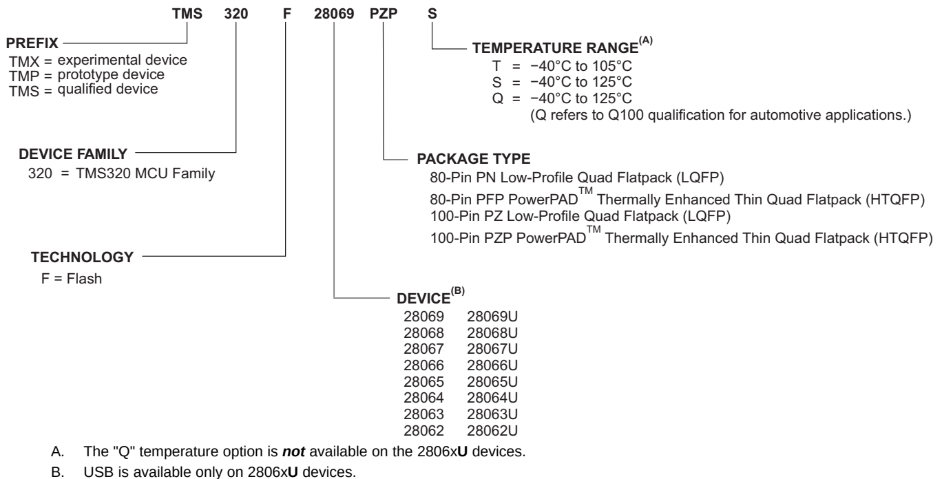
Figure 3-1. Device Nomenclature
