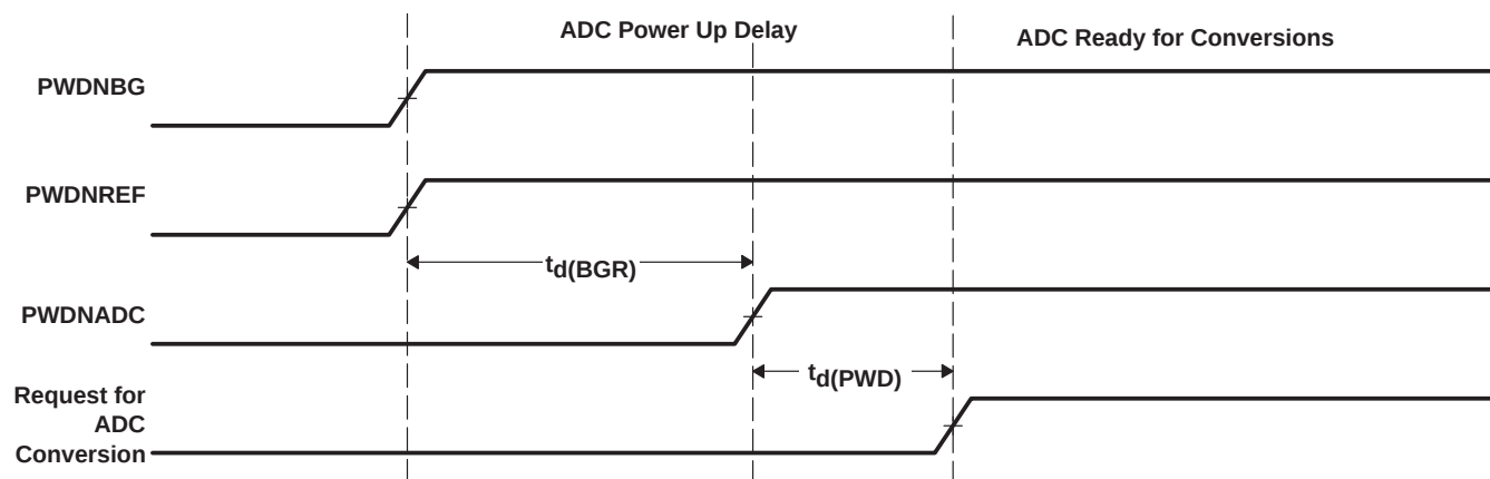
Figure 6-36. ADC Power-Up Control Bit Timing
