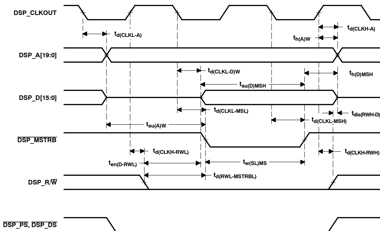
Figure 6-5. Memory Write
