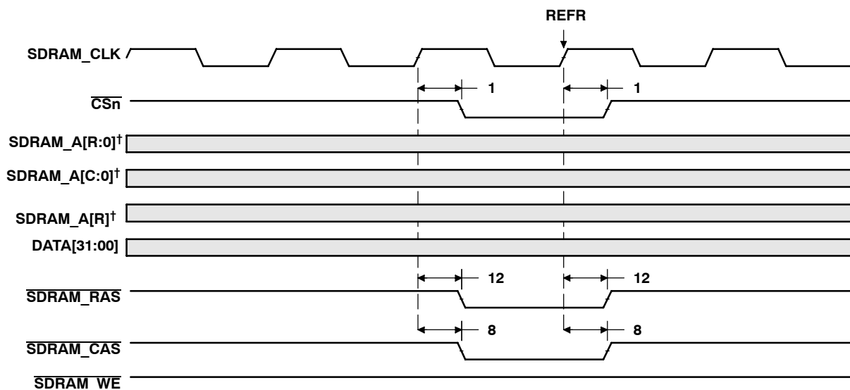
Figure 6-28. SDRAM Refresh Command
