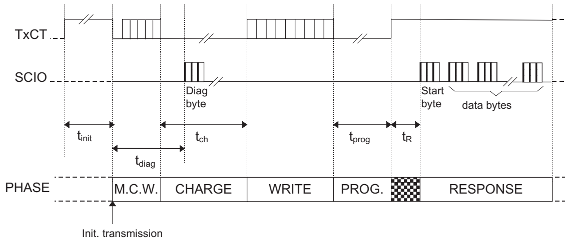
Figure 4. Write/Read Mode (Writing Into Mode Control Register)
