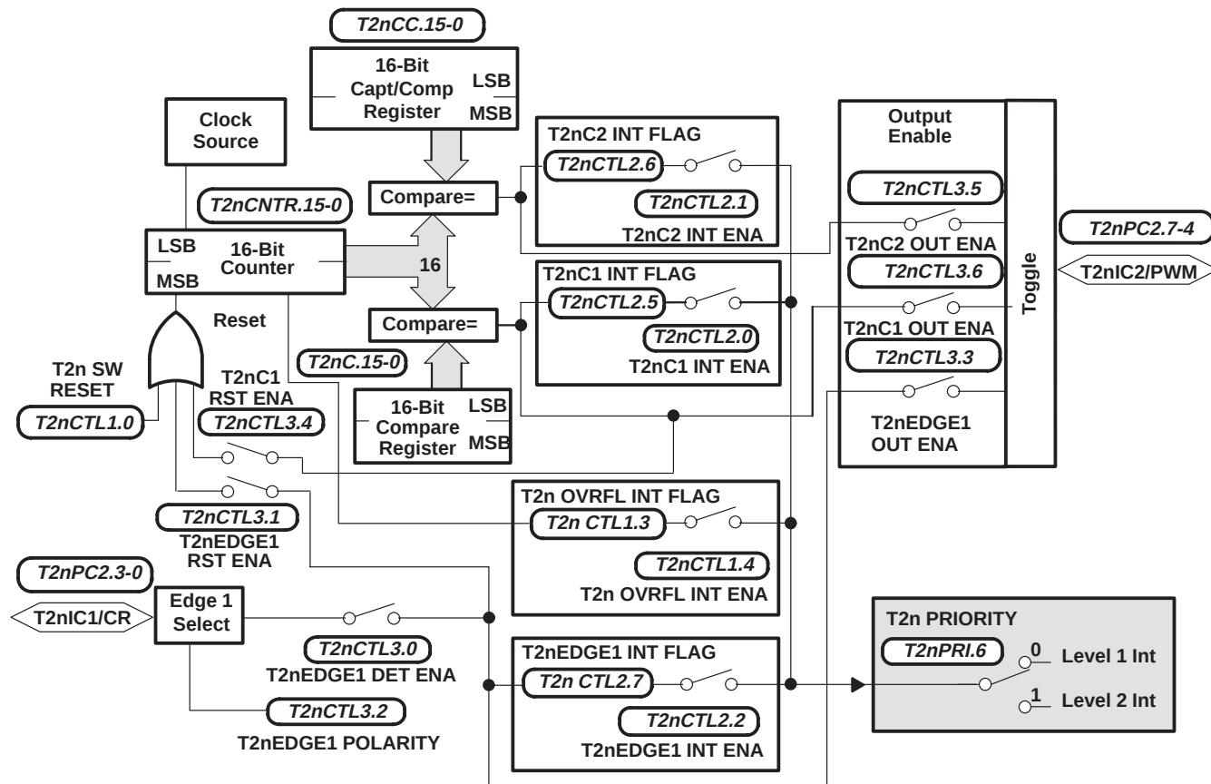
Figure 12. Dual-Compare Mode
