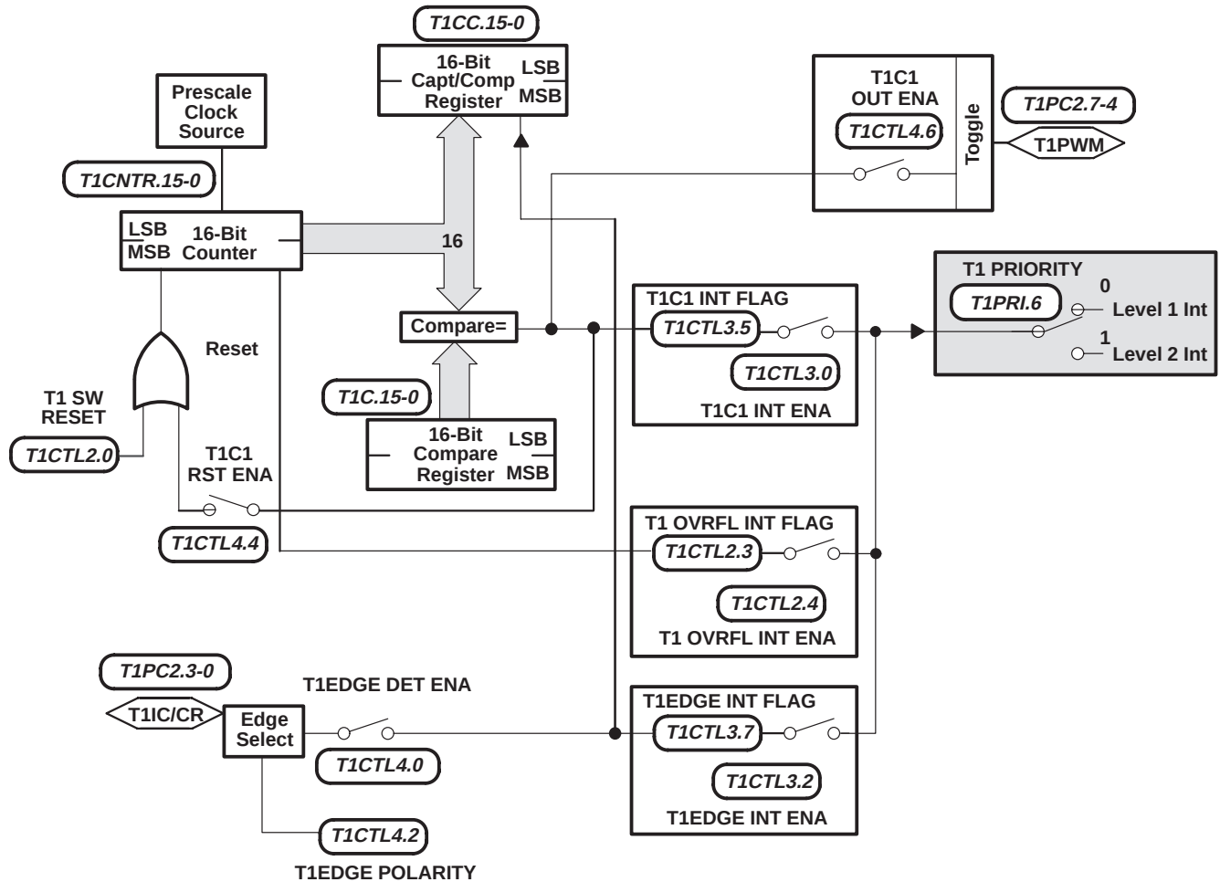
Figure 6. Capture/Compare Mode
