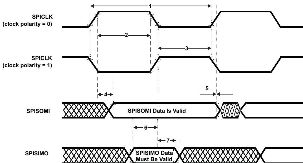
Figure 5-19. SPI Slave Mode External Timing (CLOCK PHASE = 0)
