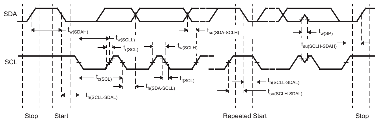
Figure 5-9. I2C Timings
