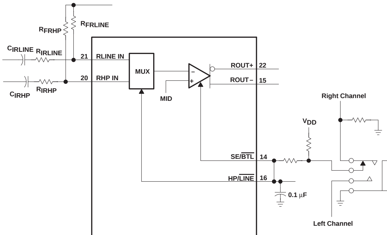
Figure 65. TPA0102 Example Input MUX Circuit
