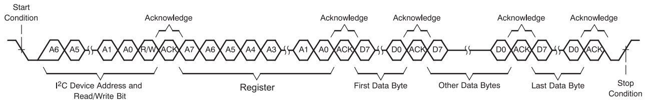
Figure 44. Multiple-Byte Write Transfer
