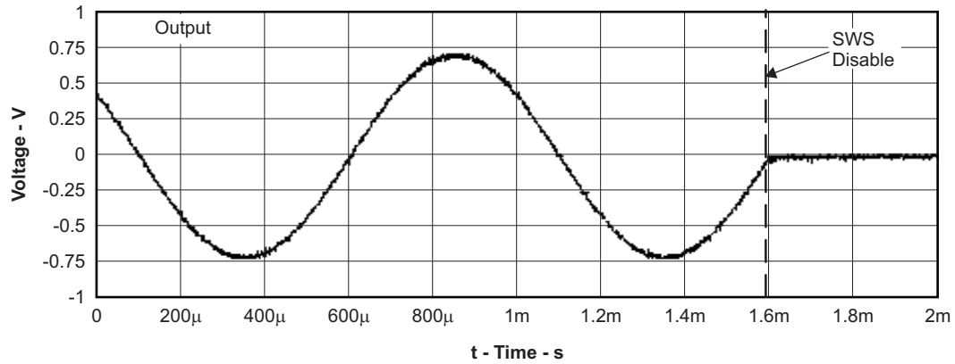
Figure 29. Shutdown Time
