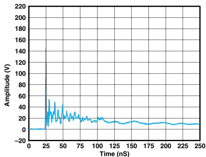
Figure 6. IEC Clamping Waveforms (8-kV Contact, Average of Ten Waveforms)
