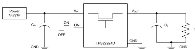
Figure 1. TYPICAL APPLICATION
