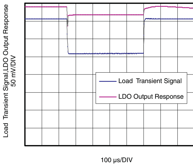
Figure 21. Load Transient
