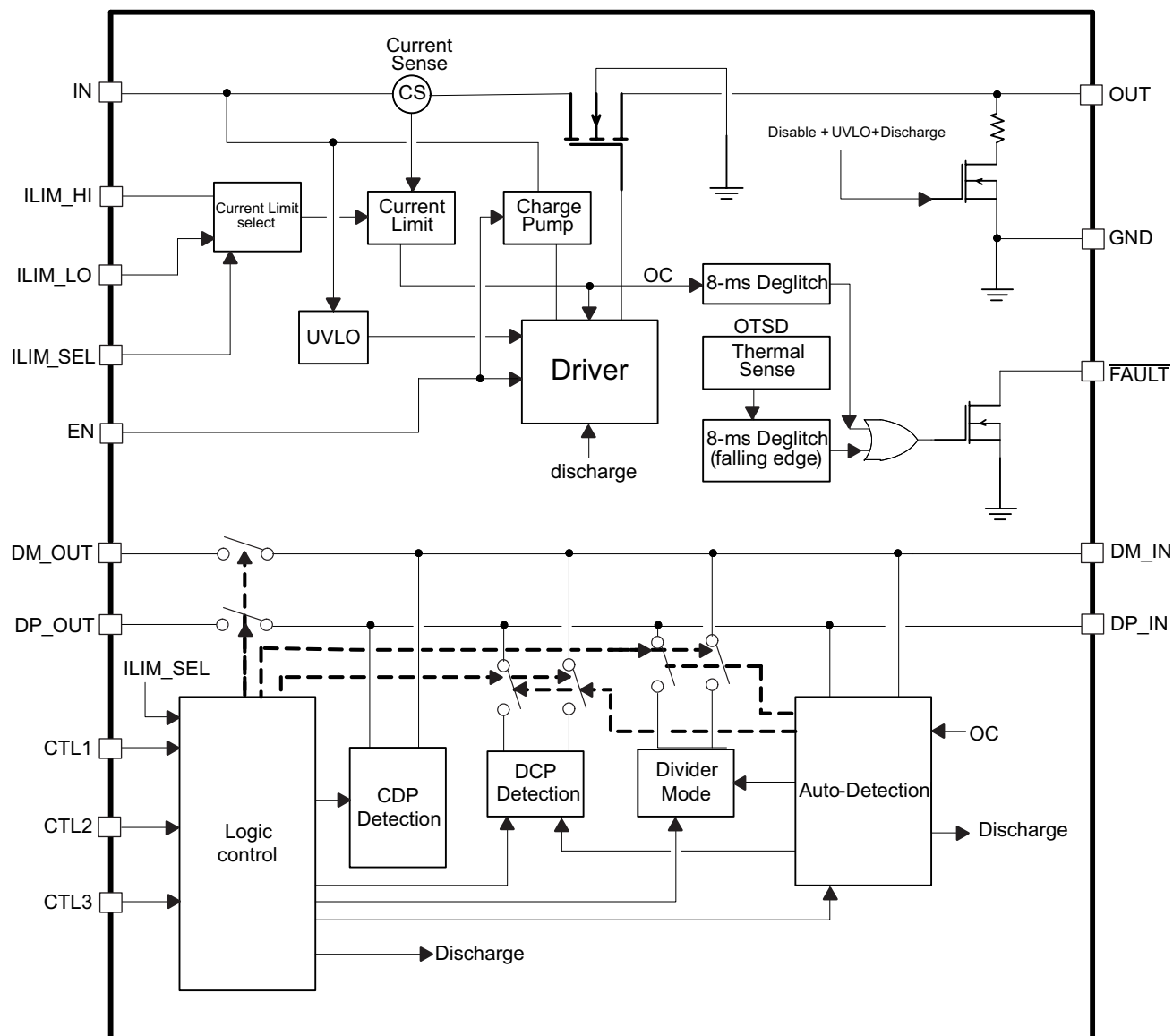
TPS2544 FUNCTIONAL BLOCK DIAGRAM
