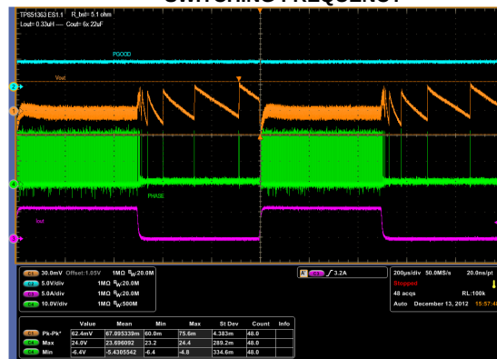
Figure 22. f = 800\text{kHz} , V_{IN} = 20\text{V} , I_{OUT} = 0-6\text{A}
