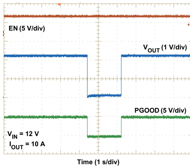
Figure 30. Over-temperature Protection
