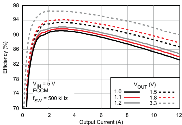
Figure 17. Efficiency vs Output Current, Inductor: HCB1175-501
