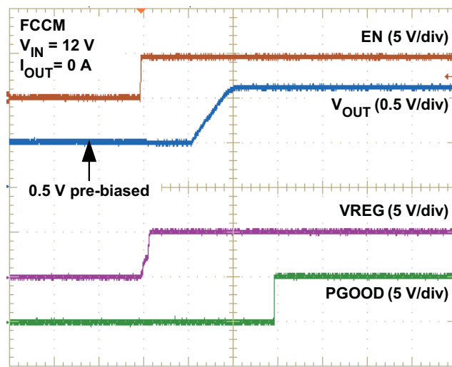
Figure 20. Pre-Bias Start-Up
