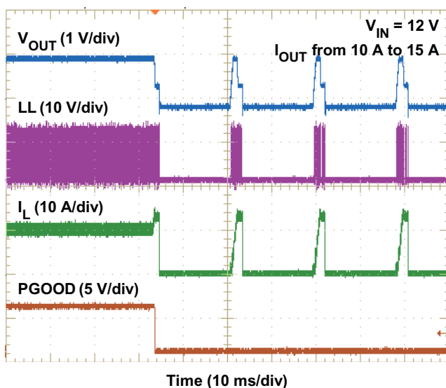
Figure 29. Overcurrent Protection
