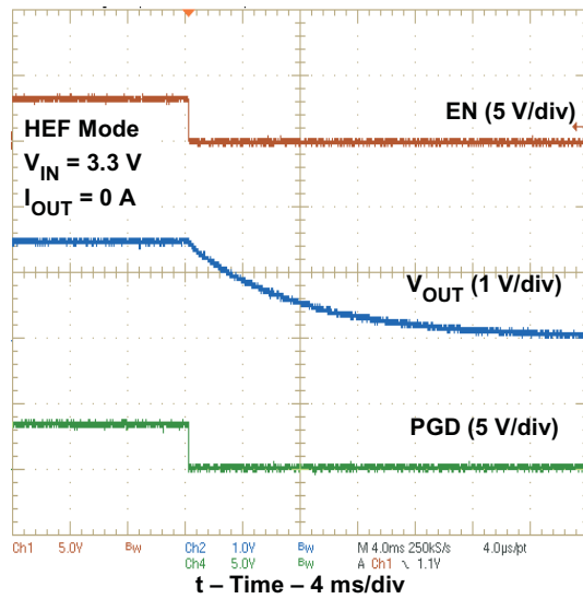
Figure 11. Soft-Stop Waveform
