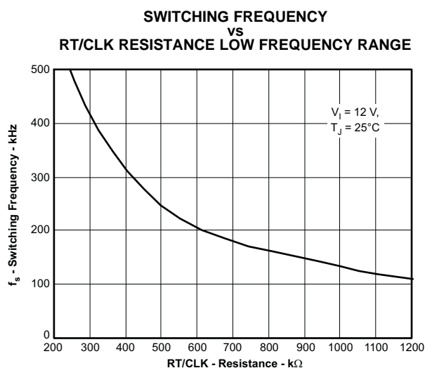
Figure 40. Low-Range RT
