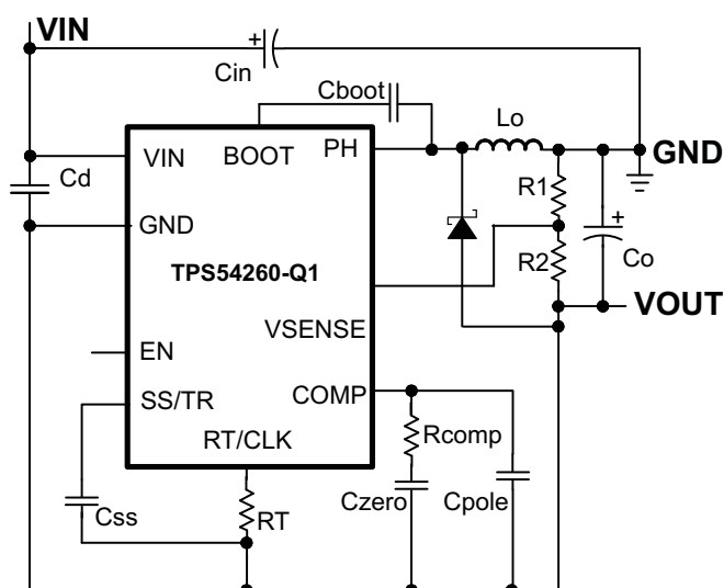
Figure 64. TPS54260-Q1 Inverting Power Supply from Application Note SLVA317
