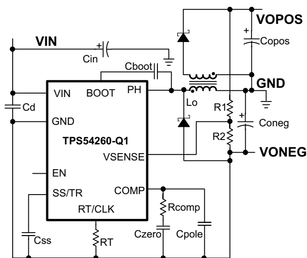
Figure 65. TPS54260-Q1 Split Rail Power Supply Based on Application Note
