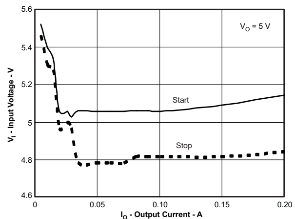
Figure 26. 5-V Start/Stop Voltage
